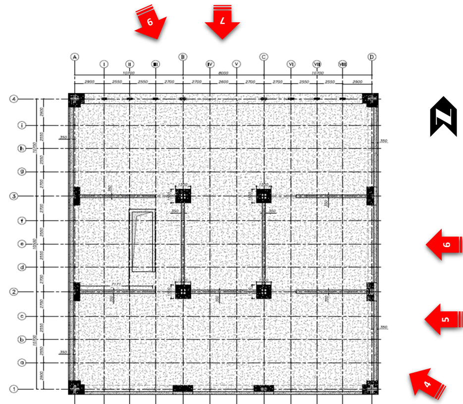
FOUNDATION & PEDESTAL FORMWORK PLAN
